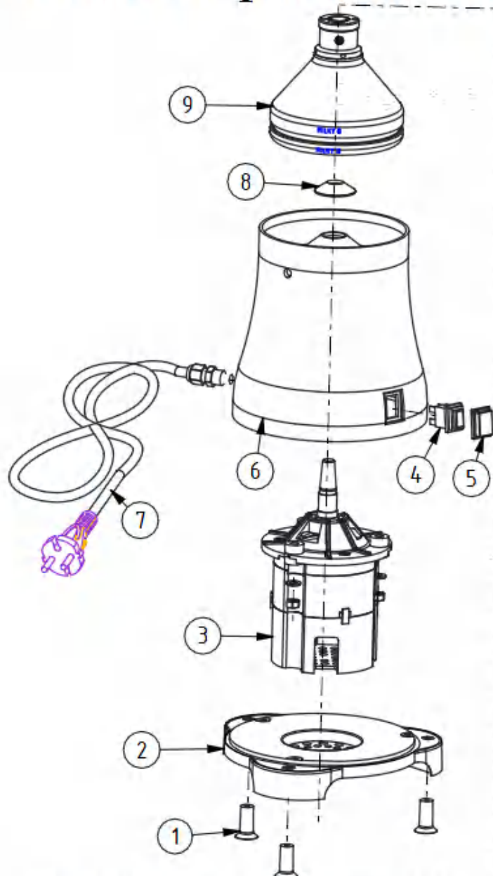
List of composing parts (Spare parts list)
