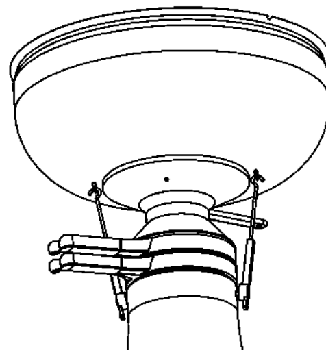
Fixing parts with rubber holder (detail).
